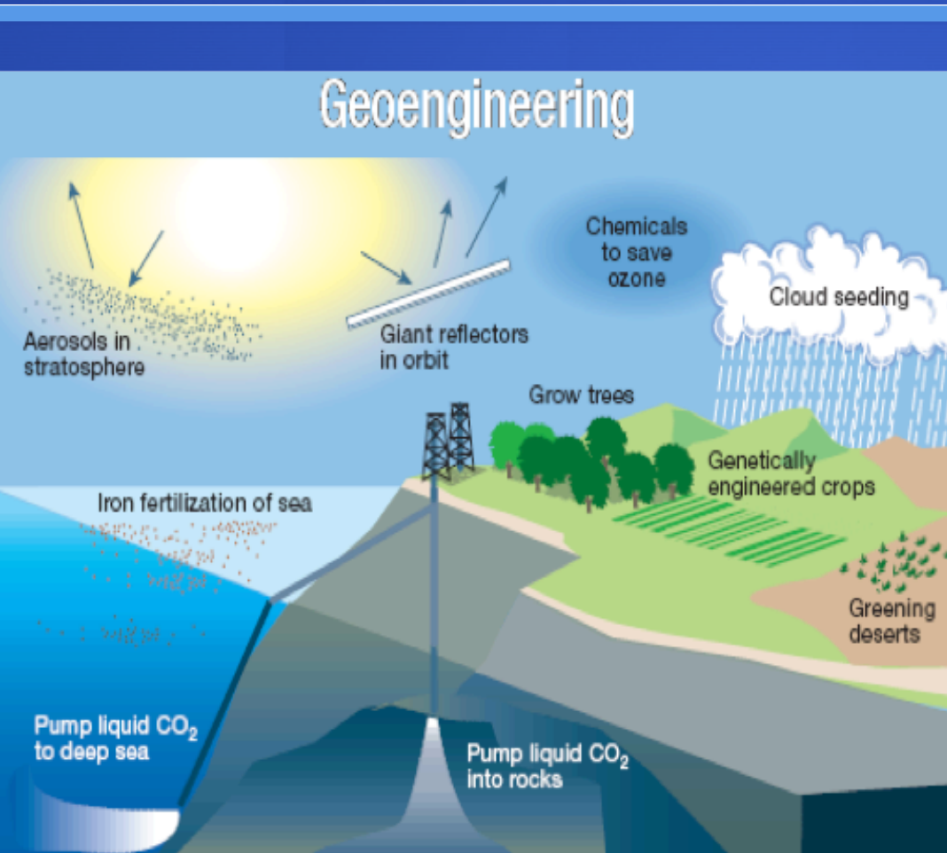
Schematic representation of various climate-engineering proposals (courtesy B. Matthews).
